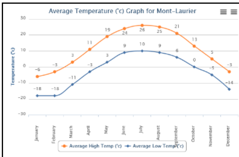
Figure 3: Average temperature graph for Mont-Laurier
