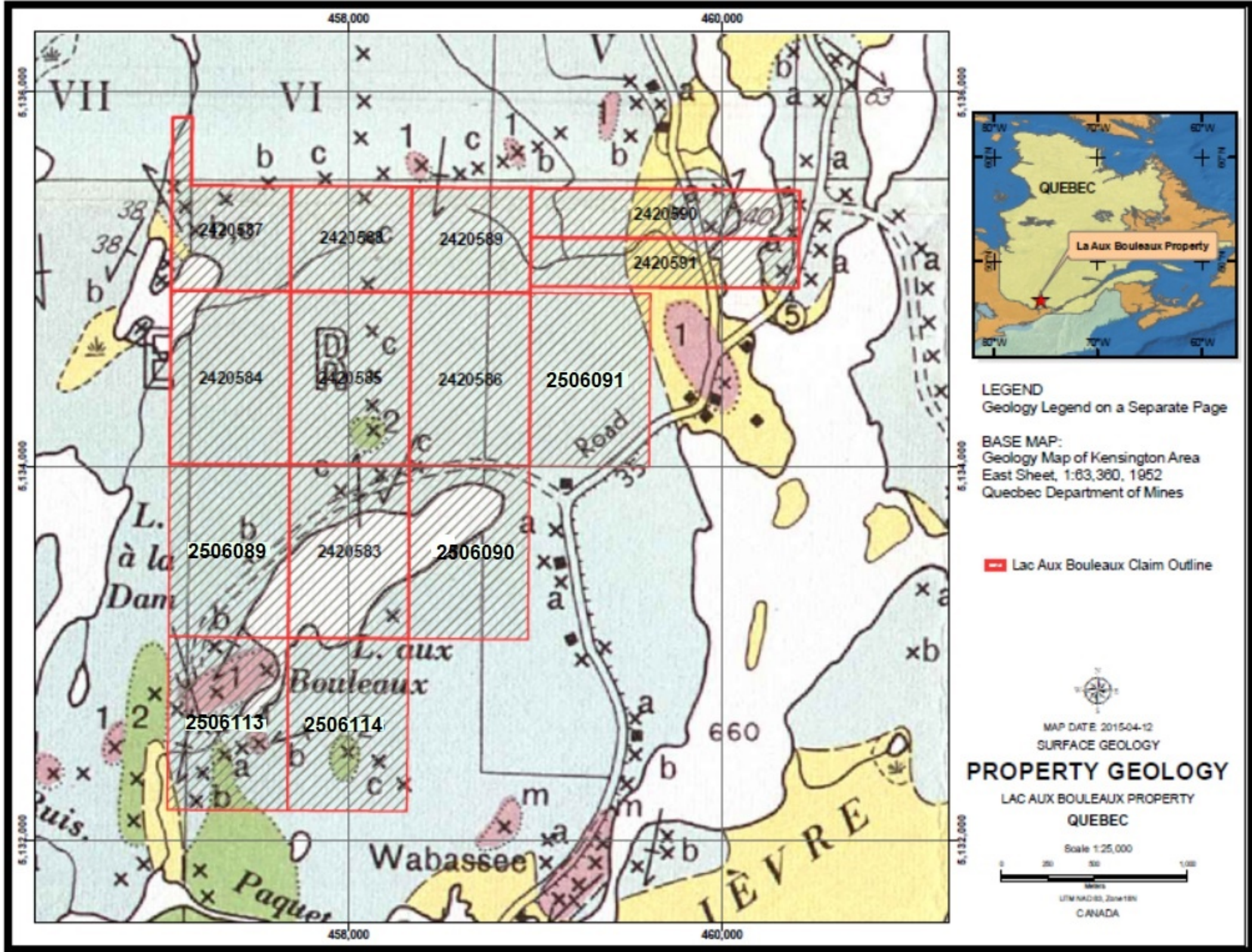
Figure 12: Property Geology
